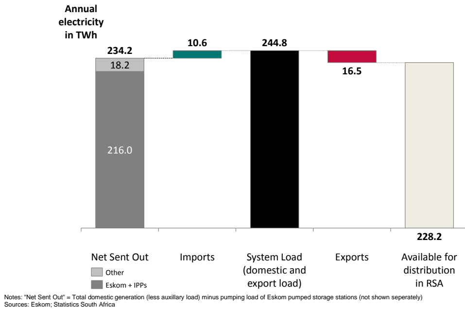
Figure 78: Current approach to determining South Africa's electricity demand
