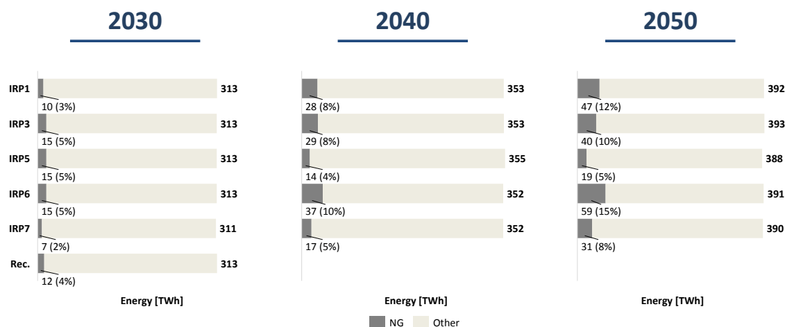
Figure 73: Summary of the role of natural gas fired generation capacity in the energy mix across Draft IRP 2018 scenarios
