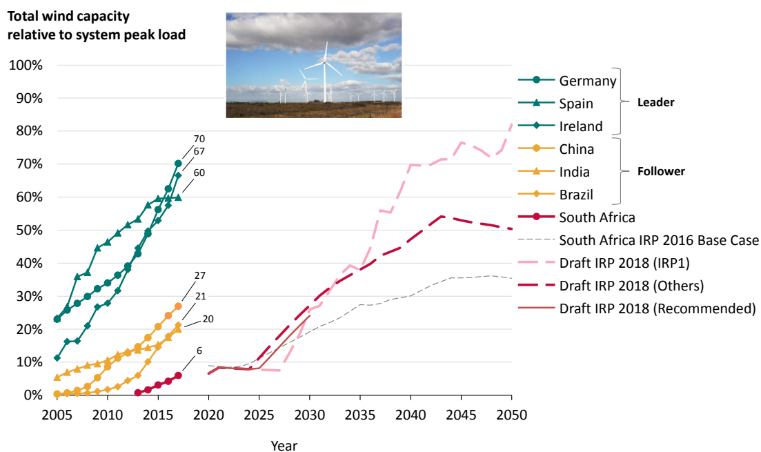
Figure 65: Global comparison of relative installed wind expected in Draft IRP 2018 scenarios relative to Leader and Follower countries
