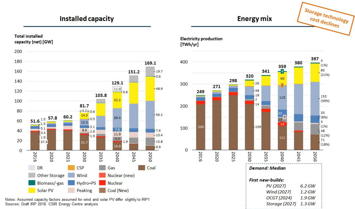
Figure 25: Installed capacity and energy mix for the stationary storage scenario
