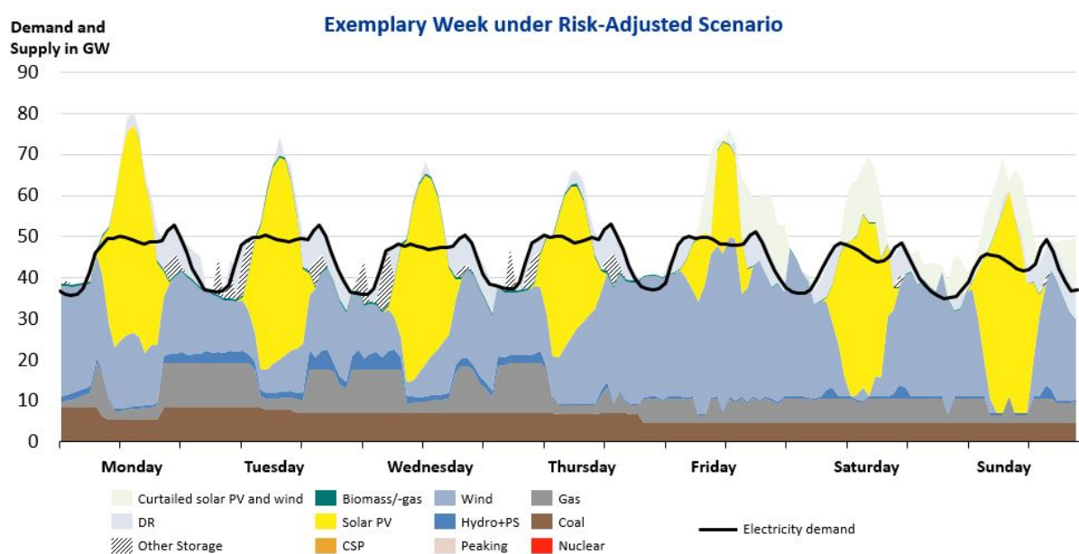
Figure 50: Risk-adjusted simulated hourly total generation and demand for an exemplary week in 2050
