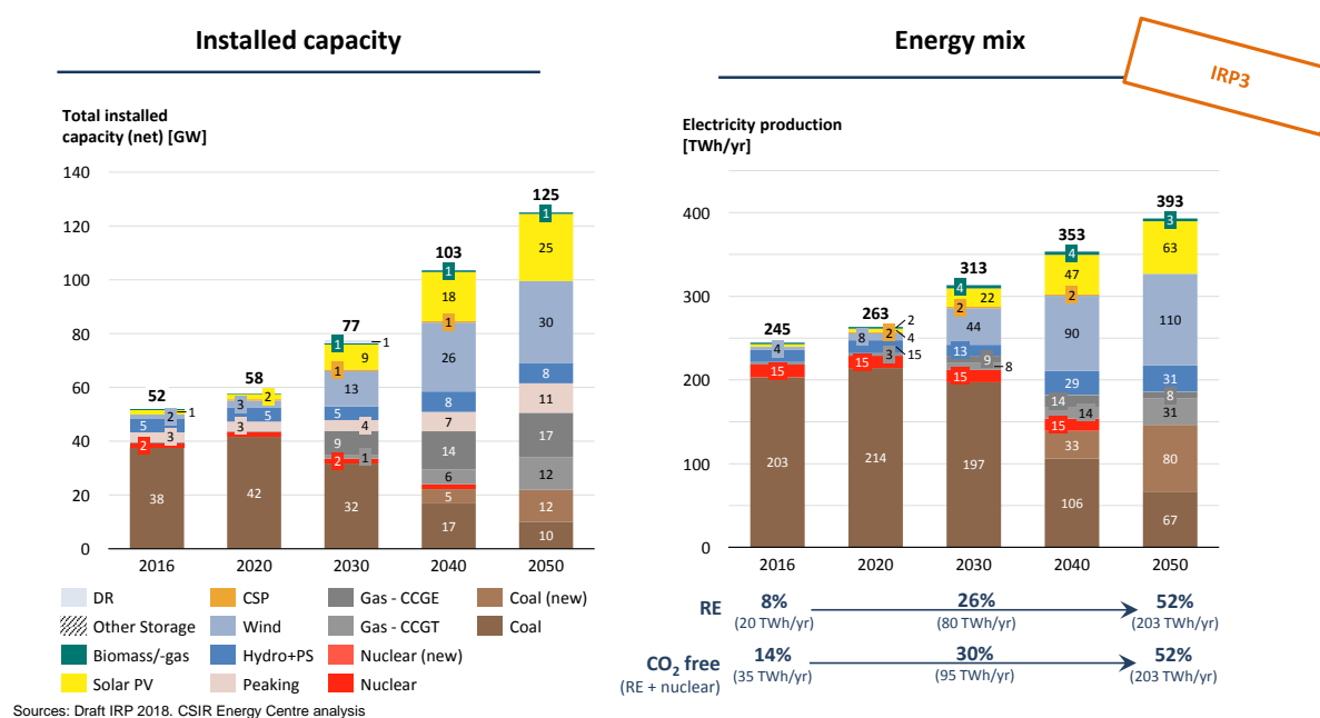
Figure 6: Installed capacity and energy mix for 2016-2050 from IRP3 in Draft IRP 2018
