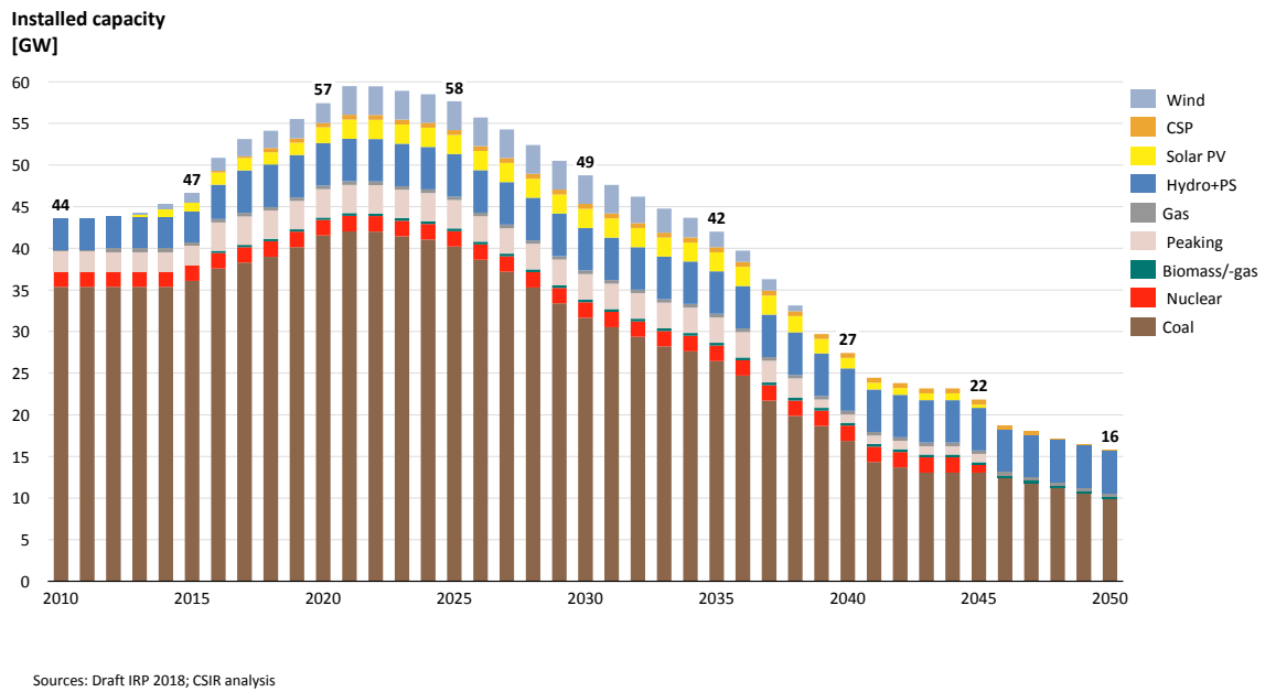
Figure 70: Total existing and under construction capacity from 1965-2050 in South Africa
