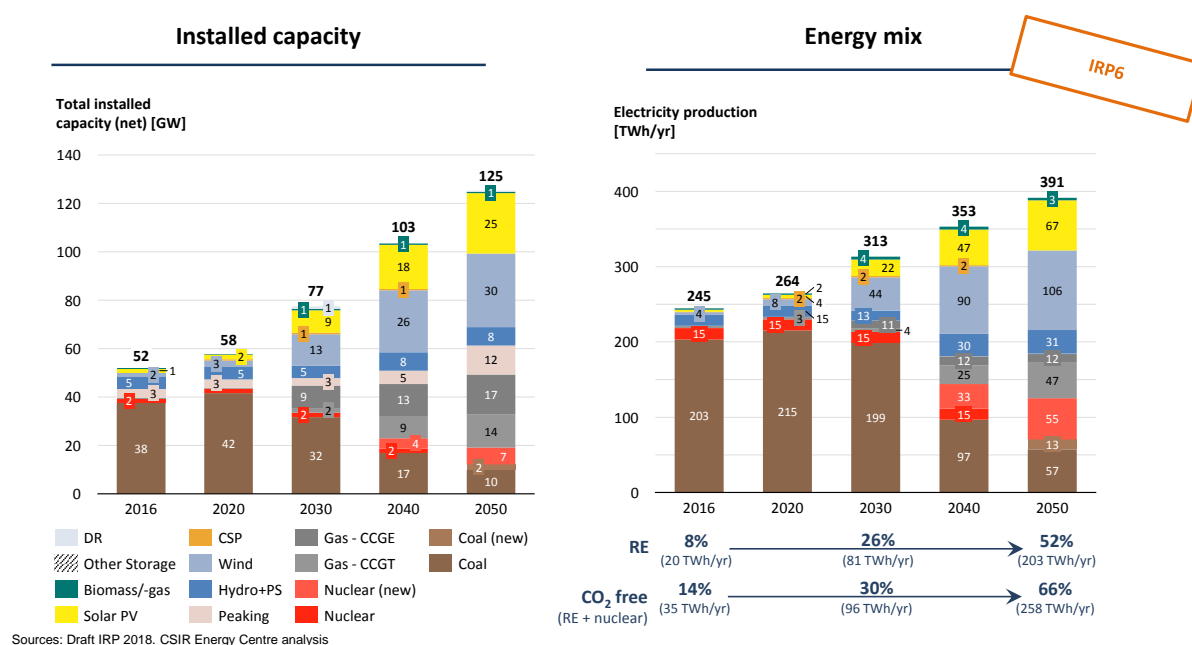
Figure 8: Installed capacity and energy mix for 2016-2050 from IRP6 in Draft IRP 2018
