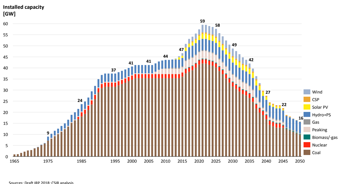
Figure 66: Total existing, under construction and committed capacity in South Africa for the period 1965-2050
