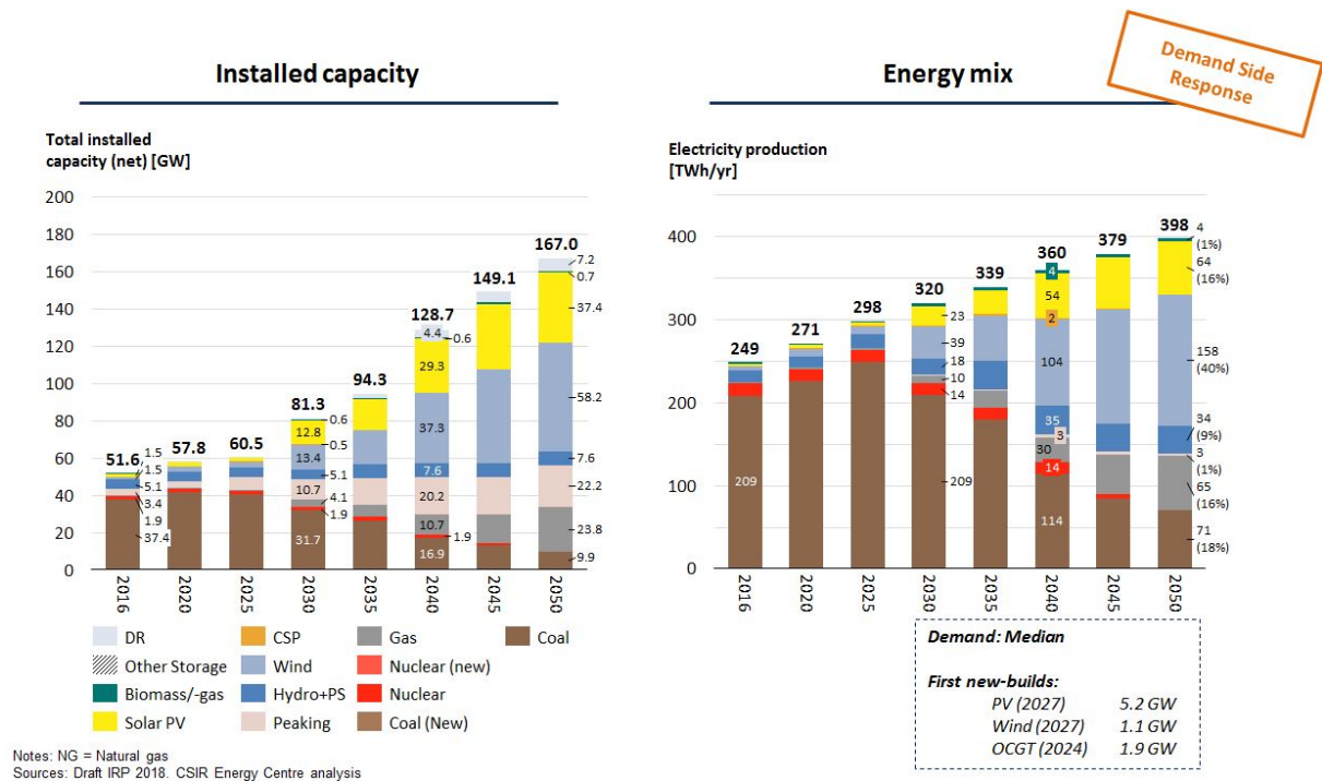
Figure 30: Installed capacity and energy mix for the DSR scenario
