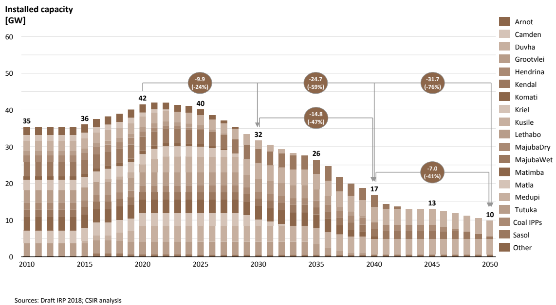
Figure 71: Existing and under construction coal capacity from 2010-2050 in South Africa
